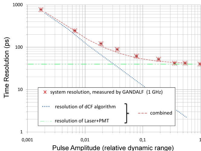
Fig. 8. Timing resolution of PMT signals generated from a Picosecond Injection Laser and measured with GANDALF.
