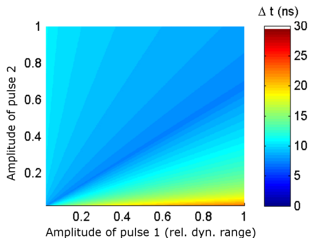
Fig. 9. Pulse separation ability of the dCFD algorithm depending on the amplitudes of the first (x-axis) and second (y-axis) pulse. The color code denotes the minimum delay between the pulses which is required for separation.
