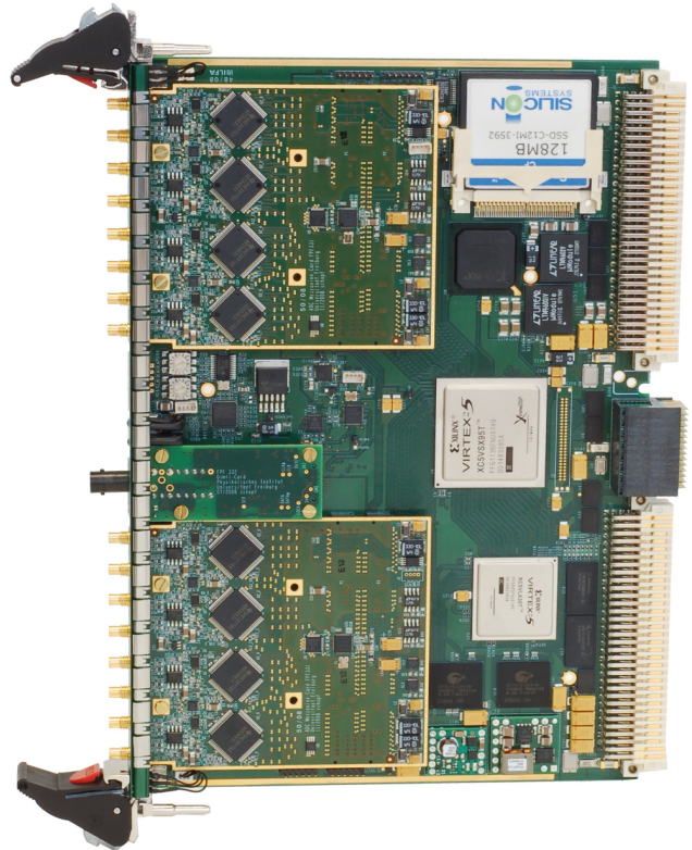
Fig. 1. Picture of the GANDALF carrier board equipped with two ADC mezzanine cards. The center mezzanine card hosts an optical receiver for the COMPASS trigger and clock distribution system.
