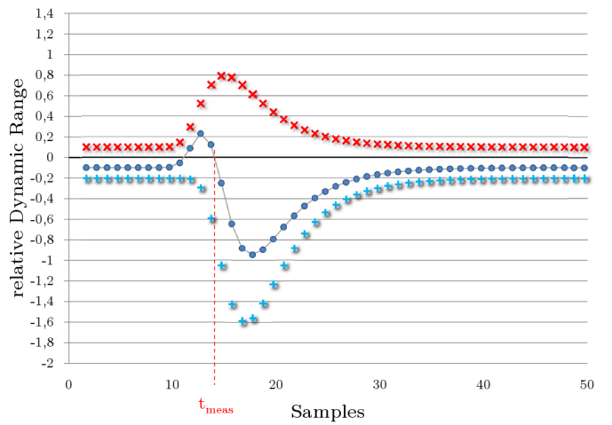
Fig. 6. Illustration of the digital constant fraction (dCF) method. The original samples ( \times ) and the delayed and inverted samples ( + ) add up to the dCF function ( \bullet ).
