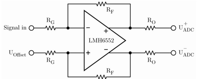
Fig. 3. Schematic of the DC-coupled analog input circuit. For each channel U_{\text{Offset}} can be set by 16-bit DACs.
